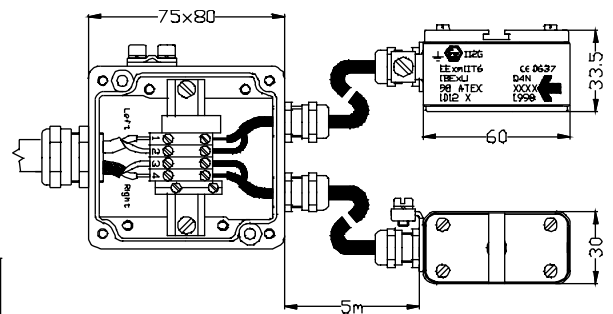
Clamp-on sensors type M4N-Ex-5-F
